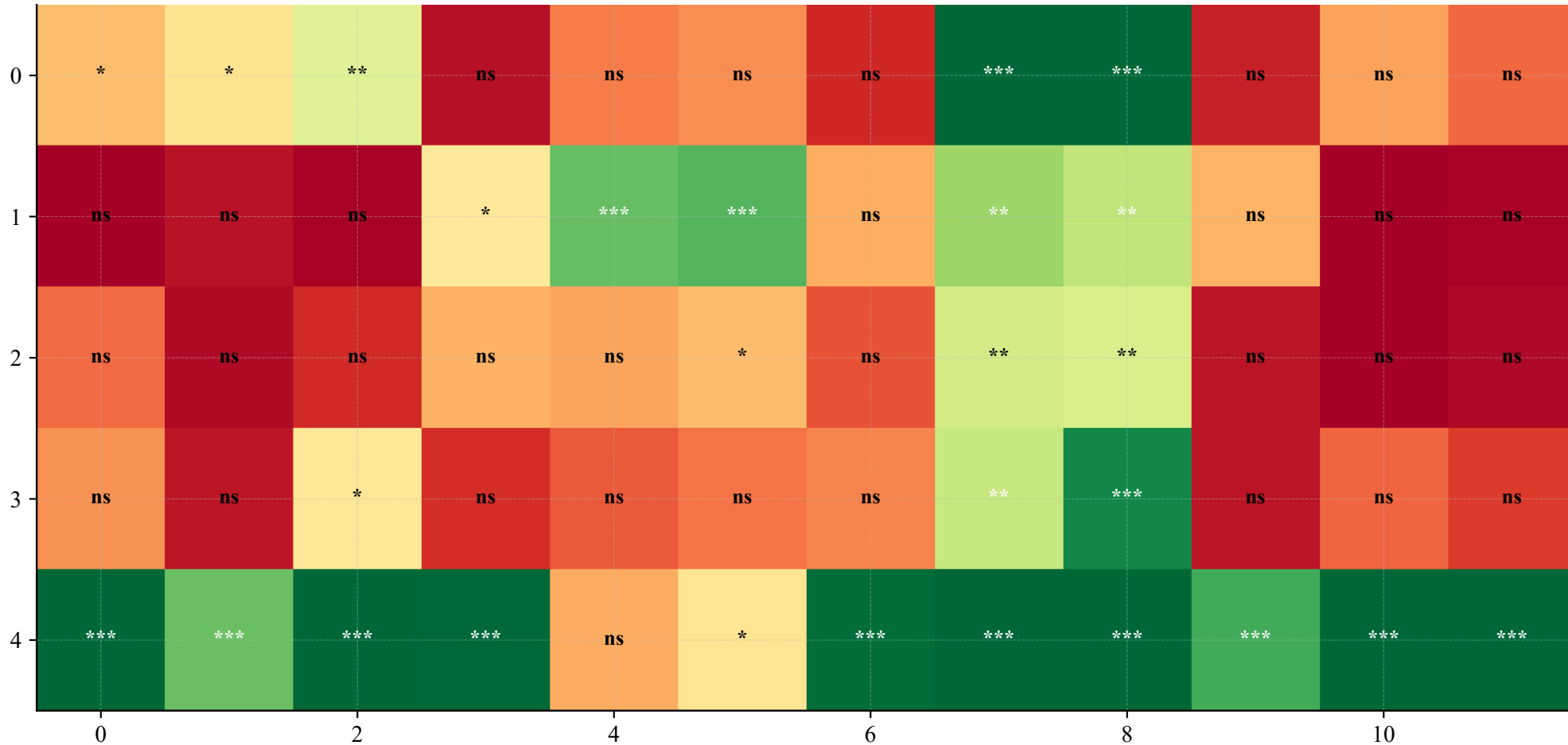
Extreme Index Wilcoxon — p-value Heatmap 1981–2014
